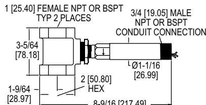
Model L6 with External Float Chamber
