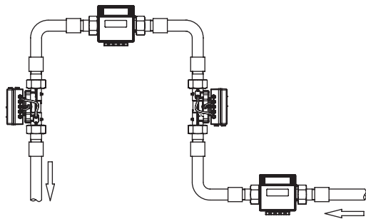
Installation Positions
