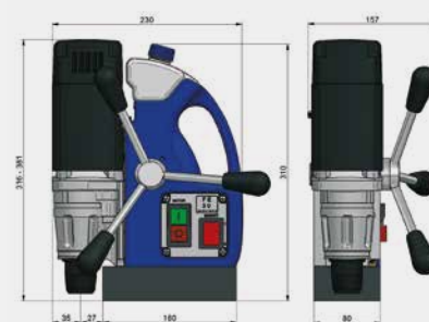
FE 30 MAGNETIC DRILLING MACHINE
