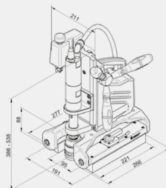
FE AIR 40 P MAGNETIC DRILLING MACHINE
