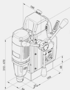
FE 100 RL X MAGNETIC DRILLING MACHINE
