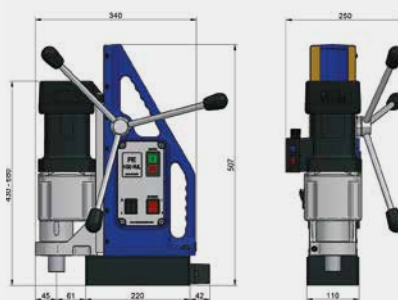
FE 100 RL X MAGNETIC DRILLING MACHINE
